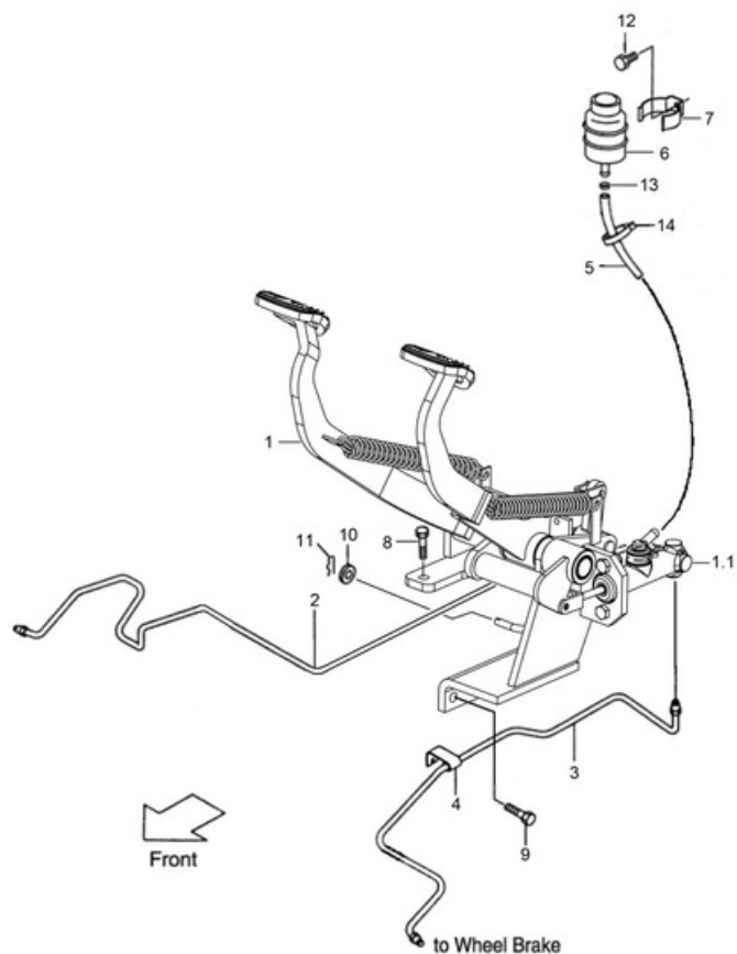
Fig.25 BRAKE PEDAL
