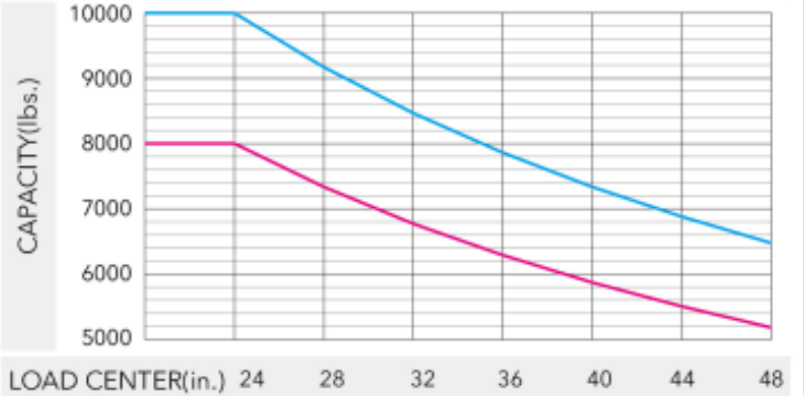
Load curve
