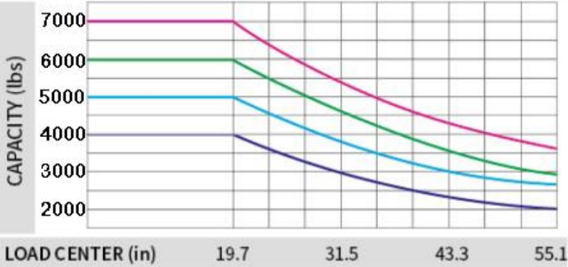
LOAD CURVE
